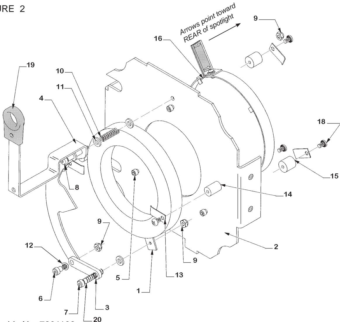
Assembly No. 7201108
