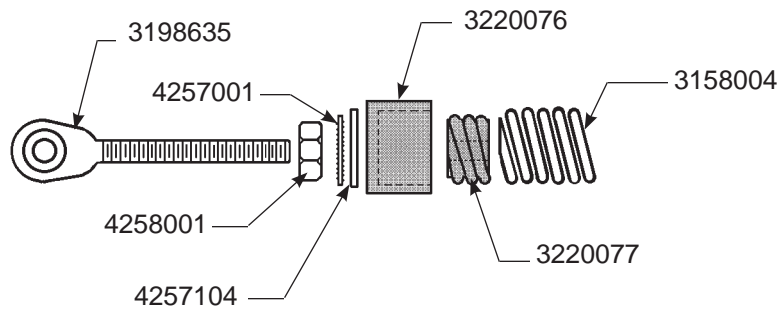
DETAIL, Item 33
